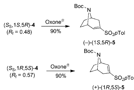
Scheme 3. Preparation of the unsaturated sulfones (–)- 5 and (+)- 5 .
