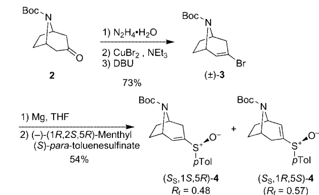
Scheme 2. Preparation of the diastereomeric unsaturated sulfoxides 4 .
