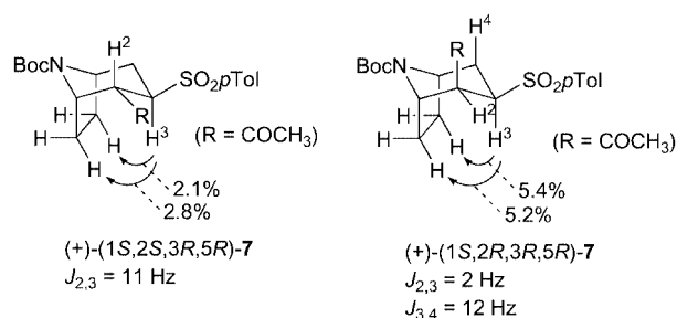
Figure 1. Relative configurations of diastereomers 7 from 1 H NMR coupling constants and NOE difference spectra.
