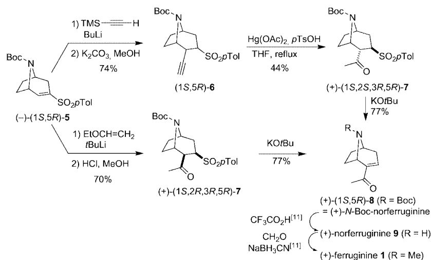
Scheme 4. Synthesis of (+)- N -Boc-norferruginine [(+)- 8 ] from unsaturated sulfone (–)- 5 .
