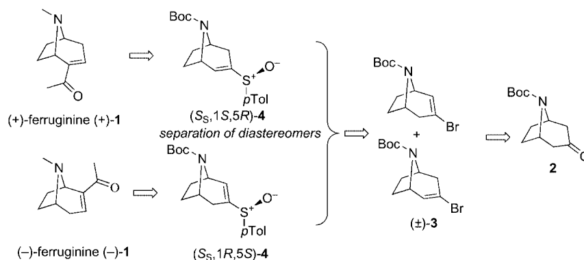
Scheme 1. Retrosynthesis of (+)- and (–)-ferruginine.
